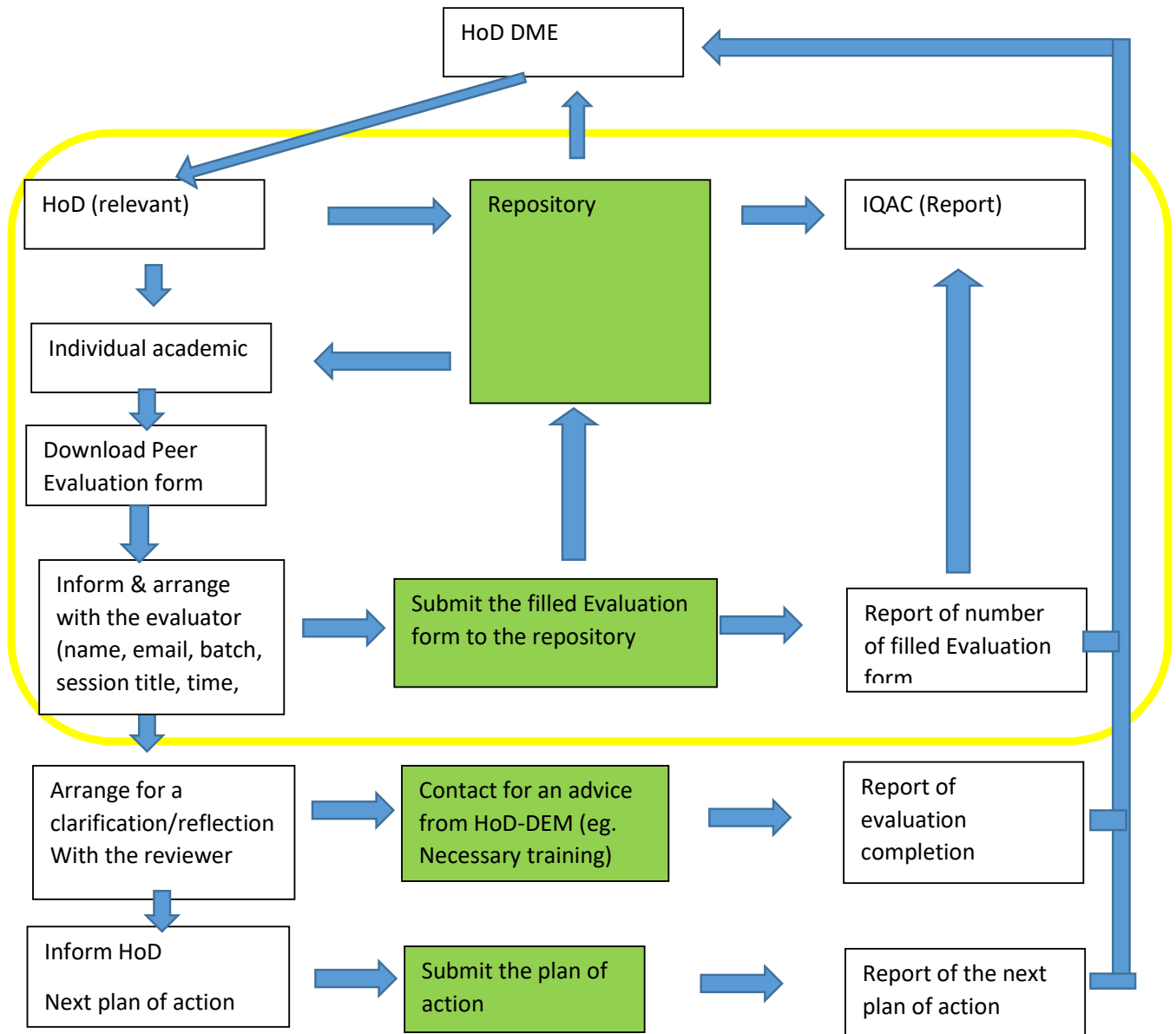
Figure 1. main event of the peer evaluation system
